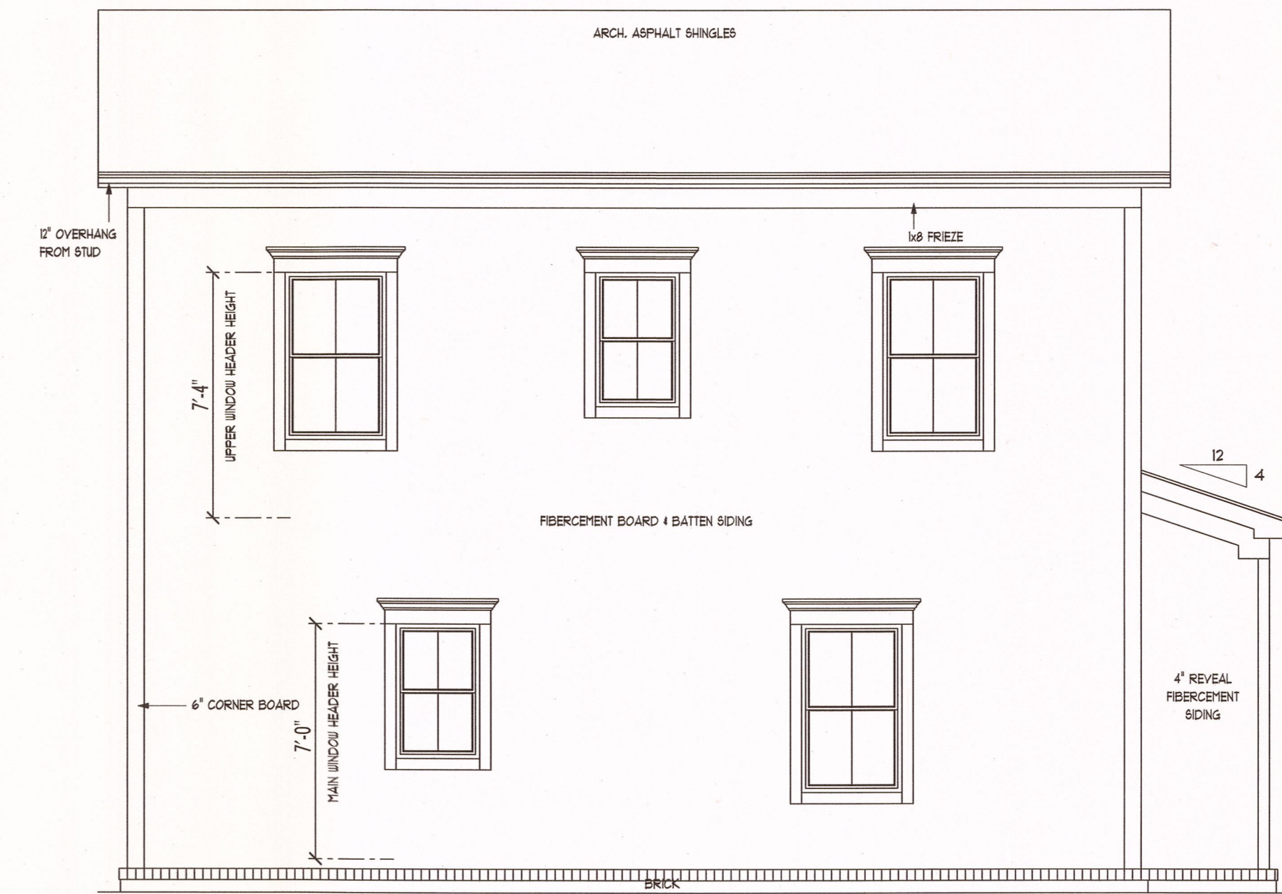
REAR ELEVATION
