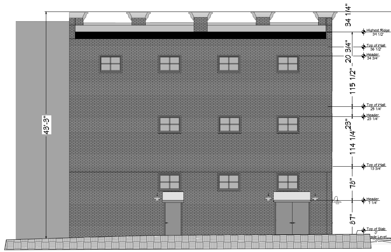
BACK ELEVATION
