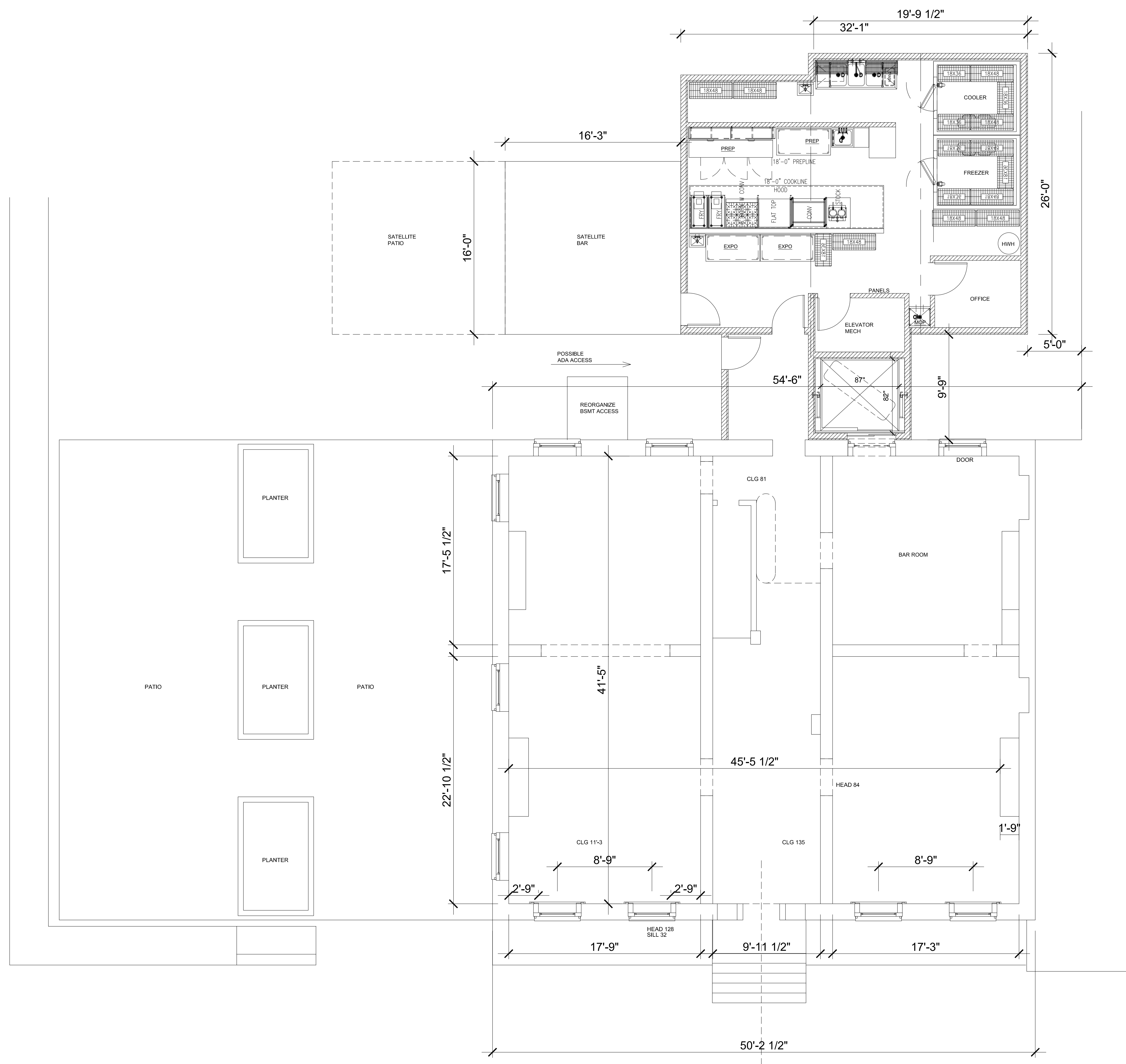
01 Main Floor Plan 1/4" = 1'-0"
